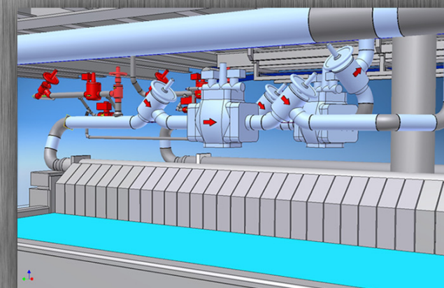
REFRIGERATION EQUIPMENT PIPING
